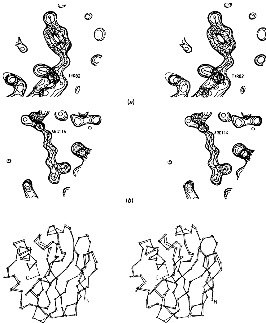
Fig. 4. Stereo pairs of two parts of the final electron density map calculated at 1.55 Å resolution showing: (a) Tyr 82 (scale = 4.80 \text{ mm } \text{Å}^{-1} ) and (b) Arg 114 (scale = 4.10 \text{ mm } \text{Å}^{-1} ) with a contour level of 0.9 \text{ e } \text{Å}^{-3} for both. A superposition is shown of 20 sections along the Z axis.
