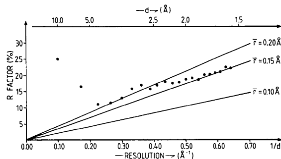
Fig. 7. Plot of R factor vs resolution after Luzzatti (1952). All reflections with F_o > 3\sigma_F were used.
