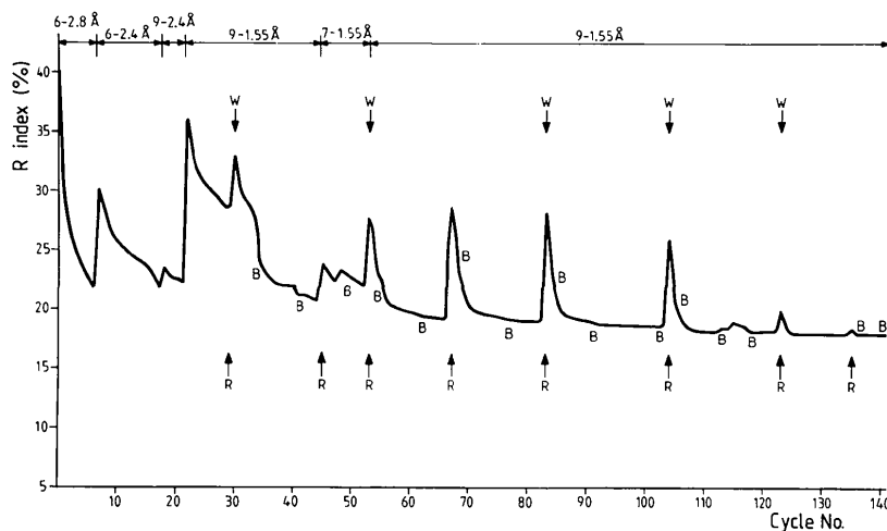
Fig. 3. Reliability factor R plotted against cycle number of the refinement. Rebuilds of the model, inclusion of solvent molecules and refinement of temperature factors are indicated, respectively, with the symbols: R , W and B . At the top of the diagram is shown the resolution range of the data included in each refinement step.
