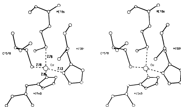
Fig. 8. Stereo computer drawing of the Cu site in pseudoazurin. The metal-to-ligand distances are given in Å.
