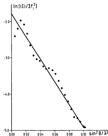
Fig. 2. The Wilson plot for the film data extending to 1.55 \text{ Å} resolution.
