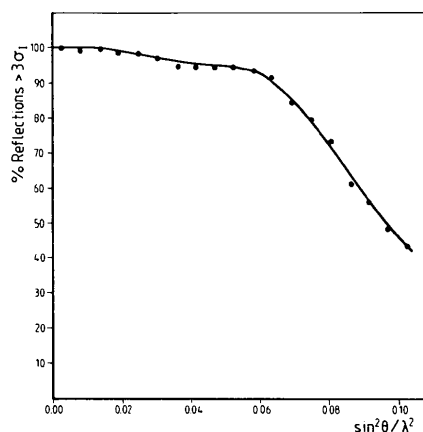
Fig. 1. Fraction of the number of reflections with intensities I > 3\sigma_I as a function of resolution.
